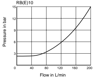
By Pass Pressure/Flow
