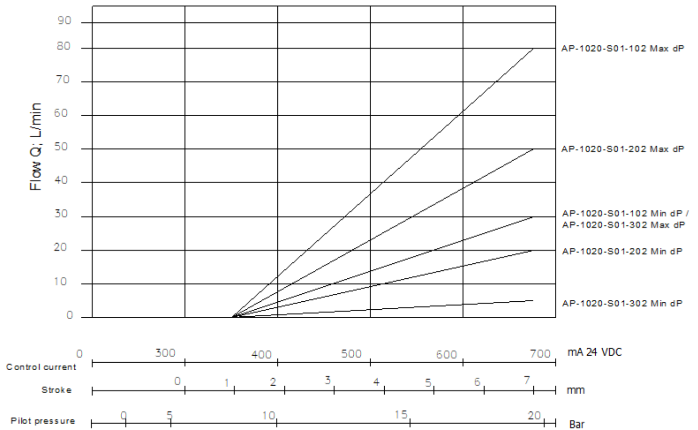
P/q curve
